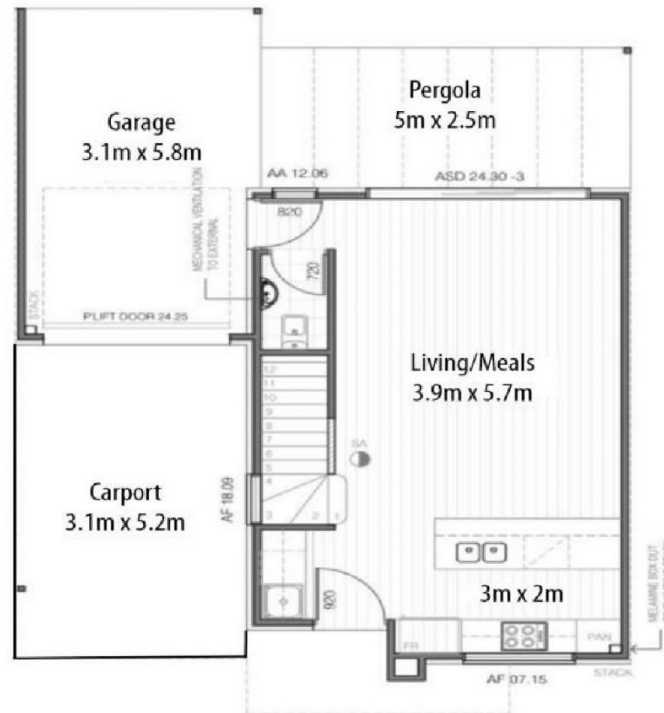
Ground Level
