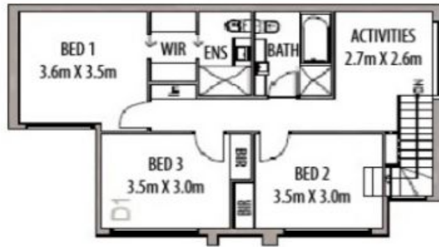
FIRST FLOORPLAN
