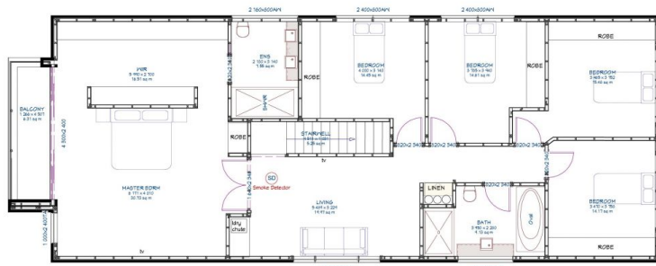
Upper Level
