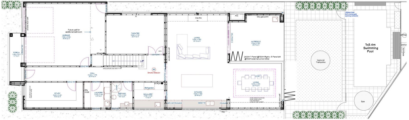
Ground Level
