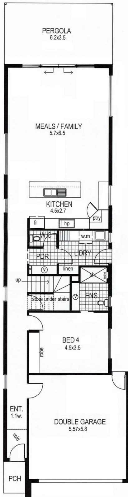
LOWER FLOOR PLAN
