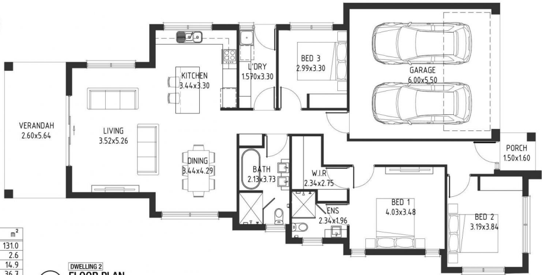
DWELLING 2 FLOOR PLAN Scale 1:100 @ A4
