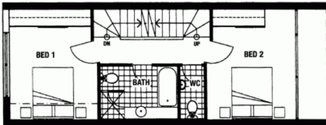
LEVEL 2
