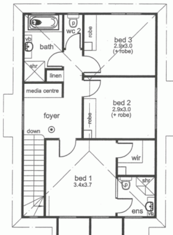
Upper Storey
