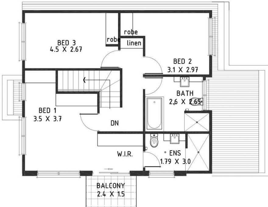
HOUSE 10 FIRST FLOOR PLAN Scale 1:100
