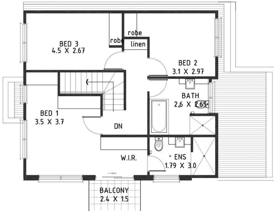
HOUSE 10 FIRST FLOOR PLAN Scale 1:100
