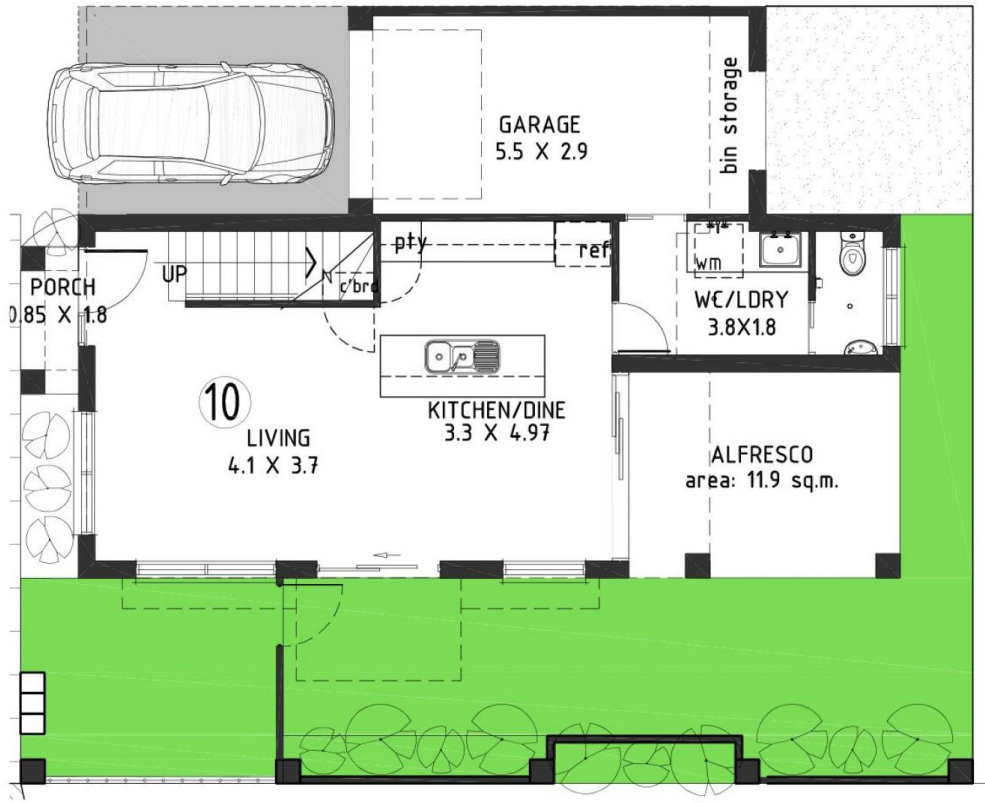
HOUSE 10 GROUND FLOOR/SITE PLAN Scale 1:100
