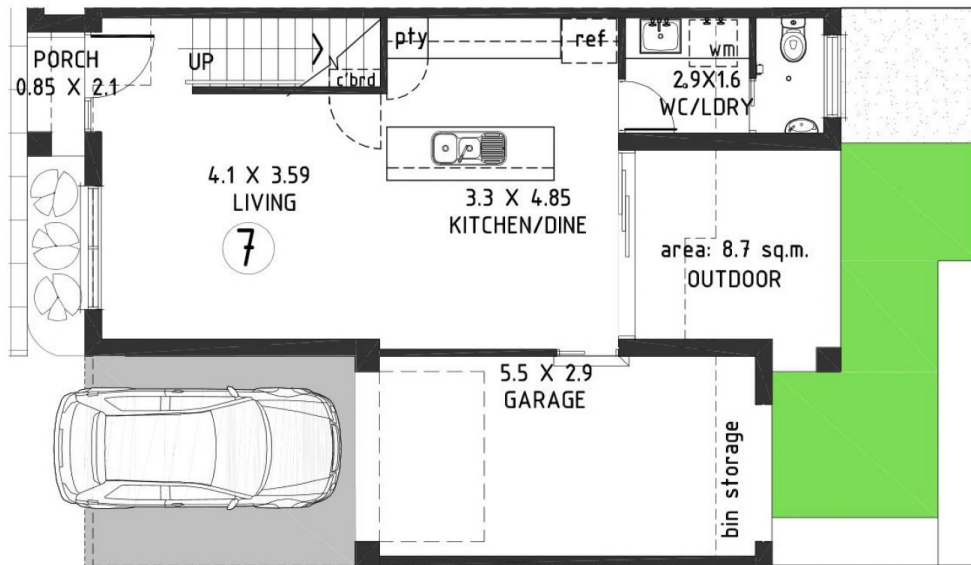
HOUSE 7 GROUND FLOOR/SITE PLAN Scale 1:100
