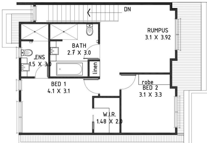
HOUSE 7 FIRST FLOOR PLAN Scale 1:100
